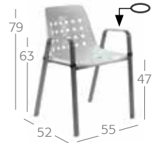
Sitzschale | Armlehnen rundoval Coque | accoudoirs ronds-ovales Seat pan | arm rests round oval 23000
